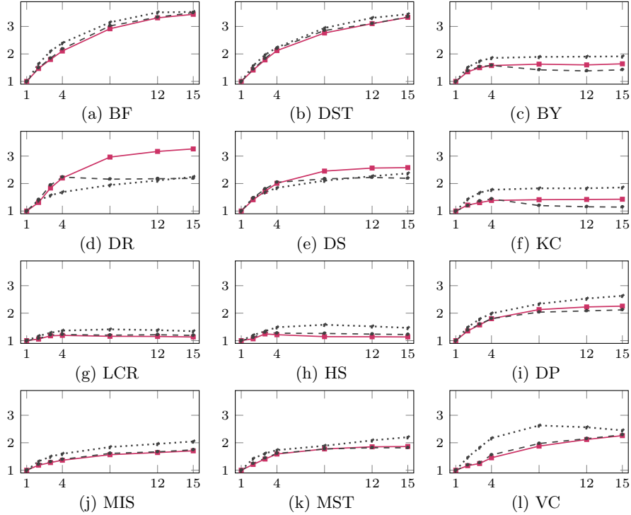
Fig. 5: Individual benchmark speedups of the NMA ( \text{---}\blacksquare\text{---} ) normalized to the baseline for varying number of compute tiles, including S_{est}^1(\cdots\cdots) , S_{est}^2(\text{---}\text{---}) : x-axis: number of compute tiles with four cores each, y-axis: relative speedup.
