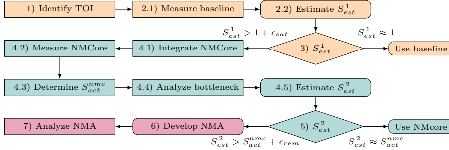
Fig. 3: Flowchart showing the steps of X-CEL
