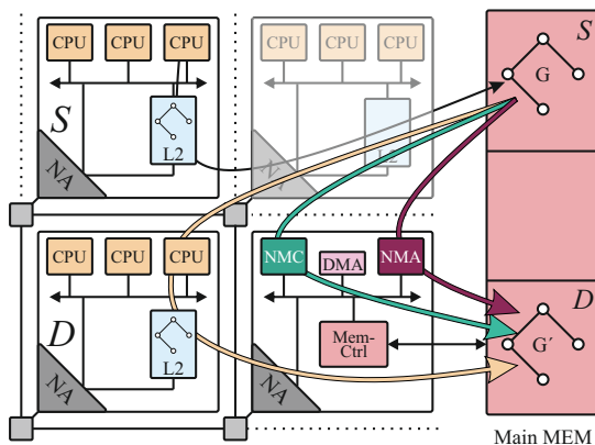
Fig. 4: Tile-based architecture.
